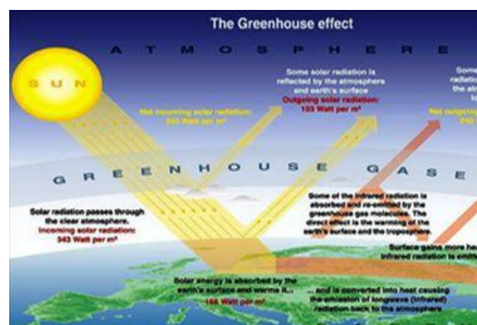
Figure 1: The greenhouse effect
