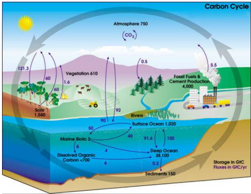
Figure 1: The Global Carbon Cycle
